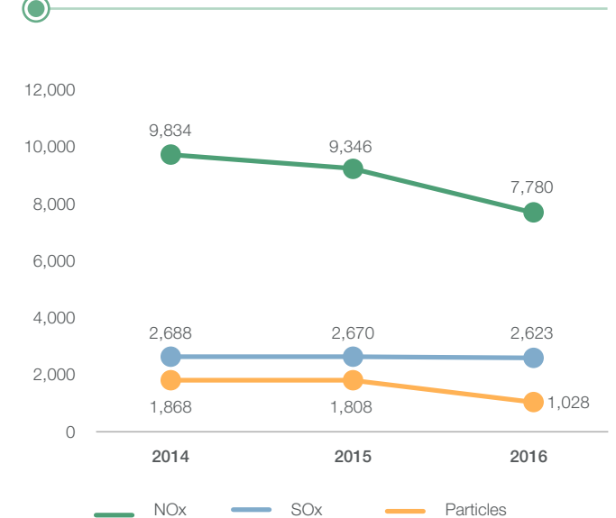
Emission of Sox, NOx and particles
